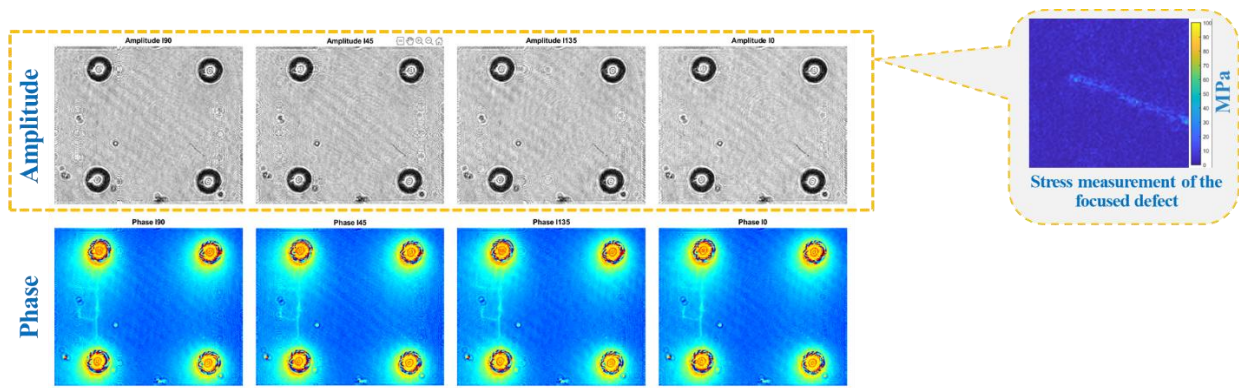
Figure 6. Depth resolved stress measurement from stress reconstruction.
