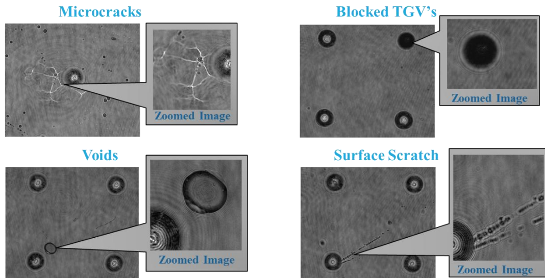
Figure 7. Defect detection.
