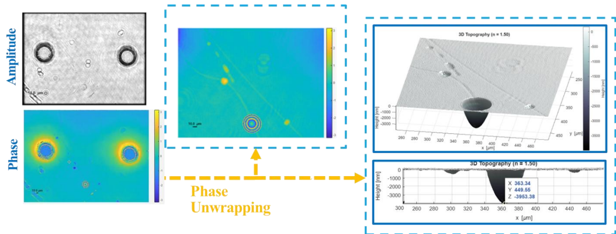
Figure 8. Defect reconstruction.
