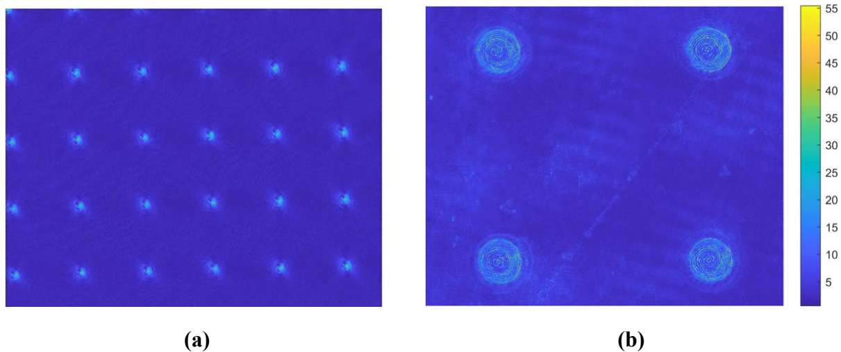
Figure 3. (a) Stress measurement of laser-modified sample (b) Stress measurement of TGV (after wet etching process). Results obtained using the proposed system.
